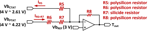
Fig. 8. Schematic of the linear adder.
