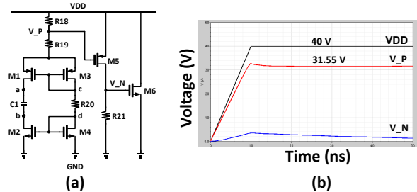
Fig. 9. Schematic of the (a) ESD protection and (b) simulated function of ESD protection.
