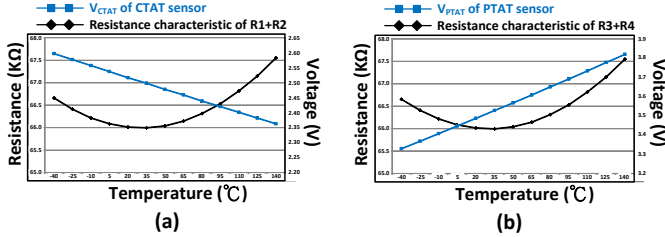
Fig. 6. Simulation of (a) V_{CTAT} and (b) V_{PTAT} vs. resistance characteristics of a silicide resistor in series with a polysilicon resistor with temperature, respectively.
